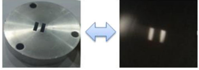
Figure 2. A radiographic image (right) of a static object (left) by the method of magnetic imaging radiography.
