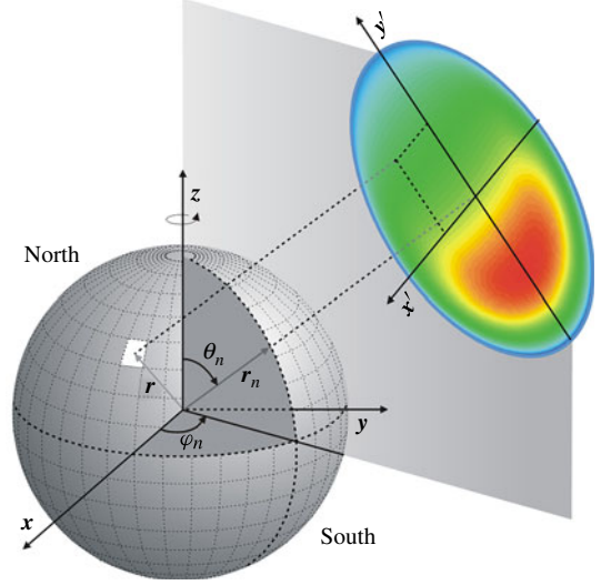
Figure 1. Spherical target and main coordinate system [O] ; vector direction \mathbf{r} of a generic surface element and versor of the n th laser beam, \mathbf{r}_n ; coordinate system [x', y'] for the n th laser intensity profile.
