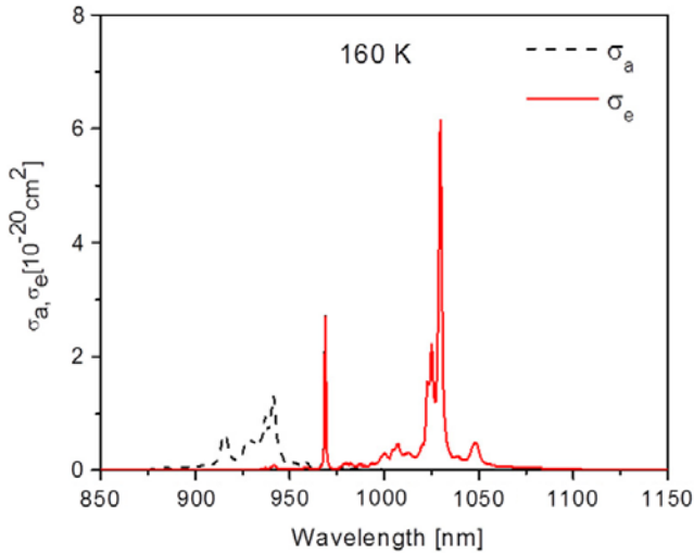
Figure 9. Measured absorption and emission cross-sections of the \text{Yb}^{3+} :YAG at a temperature of 160 K.
