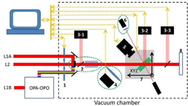
Figure 15. Schematic of the LIDT measurement station: (1) high-speed shutter, (2) beam positioning and focus, (3) beam diagnostics, (4) scattered light damage detection and fluorescence collector, (5) slow-motion camera, (6) interference damage detection; (7) XYZ tower, (8) beam dump. It uses laser pulses from Beamline A (L1A), Beamline B (L1B), and the Multi-slab (L2) laser system.
