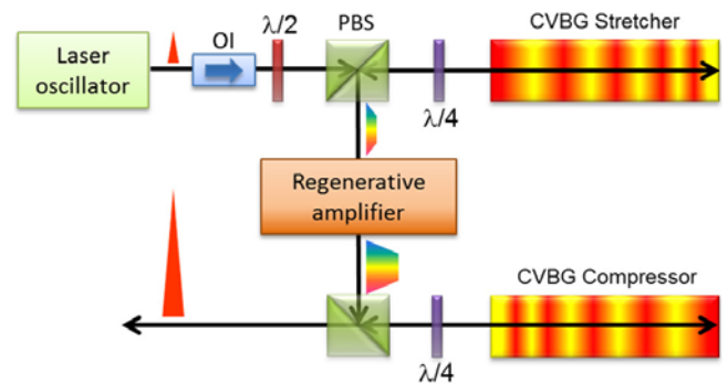
Figure 4. Schematic of the current status of Beamline C. Shown are an optical isolator (OI), \lambda/2 , \lambda/4 , PBS, and a CVBG stretcher and compressor.
