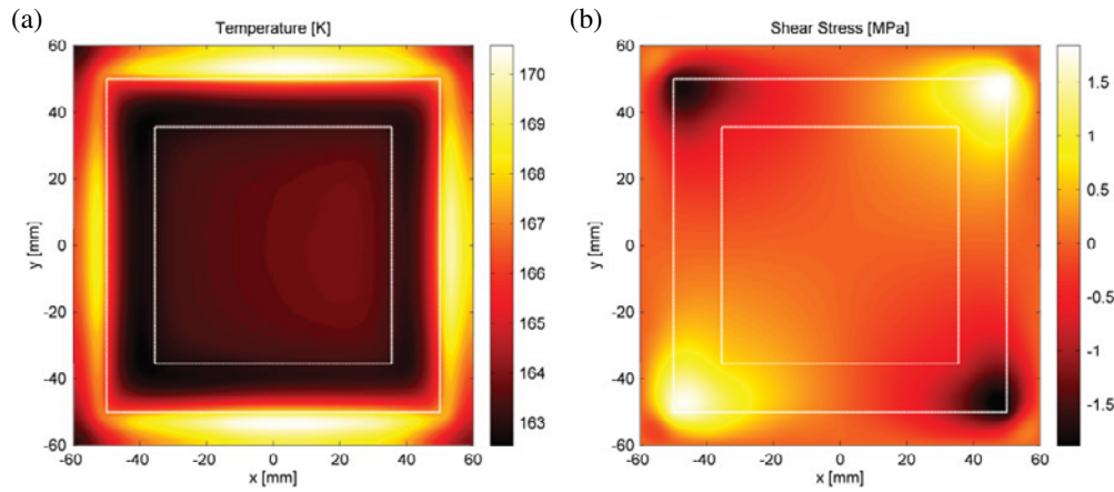
Figure 10. (a) Transverse distribution of temperature and (b) transverse distribution of the xy stress component in a longitudinal cut in the center of the laser slab.
