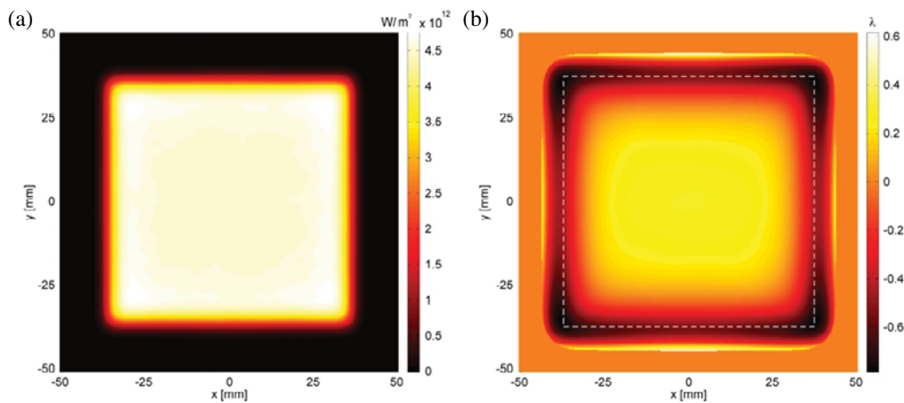
Figure 12. (a) Beam profile and (b) OPD of the beam at the output of the 100 J multi-slab system calculated in MIRÓ. Dashed square indicates the position of the laser beam.
