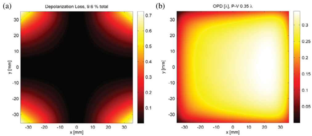
Figure 11. (a) Depolarization of the beam at the output of the amplifier (after four passes through six laser slabs) caused by stress-induced birefringence. (b) Stress- and temperature-induced OPD after a single pass through the laser head (after one pass through six laser slabs).
