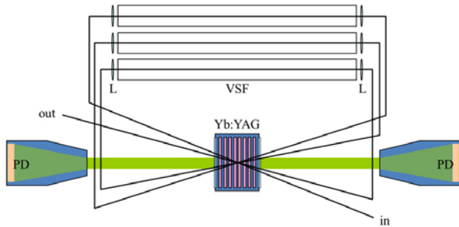
Figure 7. Schematic of the 100 J cryogenic multi-slab amplifier. It consists of Yb:YAG, lenses (L), VSF, and PD.
