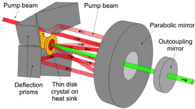
Figure 1. Schematic of the thin-disk cavity consisting of a parabolic mirror focusing the pump beam onto the thin-disk crystal. Multiple passes of the pump beam are made by means of deflection prisms. The cavity for laser beam extraction is formed by the thin-disk crystal and the outcoupling mirror [14].
