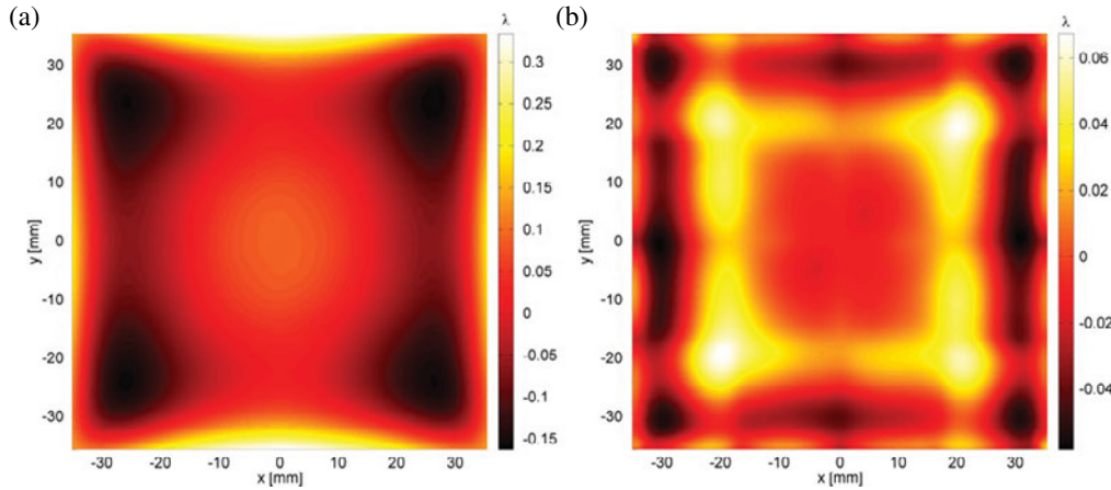
Figure 13. (a) Output OPD calculated in MIRÓ and shown in Figure 12(b) after subtraction of tilt and defocus. (b) Residual OPD after correction by the deformable mirror with 36 actuators.
