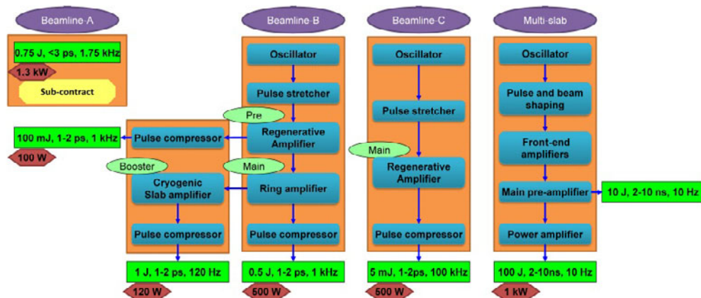
Figure 2. Overview of the HiLASE beamlines.
