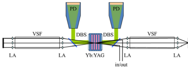
Figure 6. Schematic of the 10 J cryogenic multi-slab amplifier. It consists of \text{Yb}^{3+} :YAG ceramic slabs in the laser head (Yb:YAG), dichroic beam splitters (DBSs), lens arrays (LAs), vacuum spatial filters (VSFs), and homogenized pump diode laser modules (PDs).
