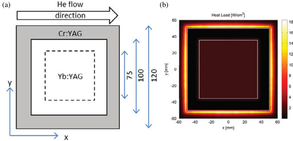
Figure 8. (a) Schematic of the laser slab with dimensions in mm, dashed line shows the spot of the pump beam in the \text{Yb}^{3+} :YAG part of the slab that is clad by \text{Cr}^{4+} :YAG. (b) Transverse heat load of the slab used for the calculations (assumed constant in the longitudinal direction).
