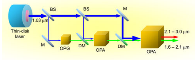
Figure 16. Schematic of the mid-IR parametric generator and amplifier. It consists of the thin-disk laser system, beam splitters (BS), mirrors (M), dichroic mirrors (DM), an OPG, and OPA.
