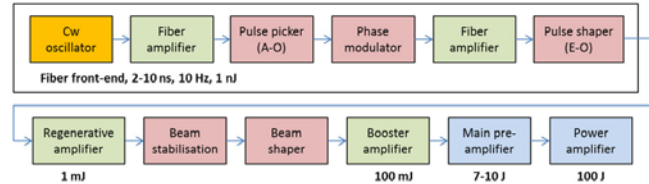
Figure 5. Schematic of the 100 J multi-slab laser system. The numbers represents the energy after the respective element.
