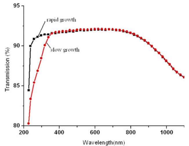
Figure 3. Transmission spectra of KDP crystals.
