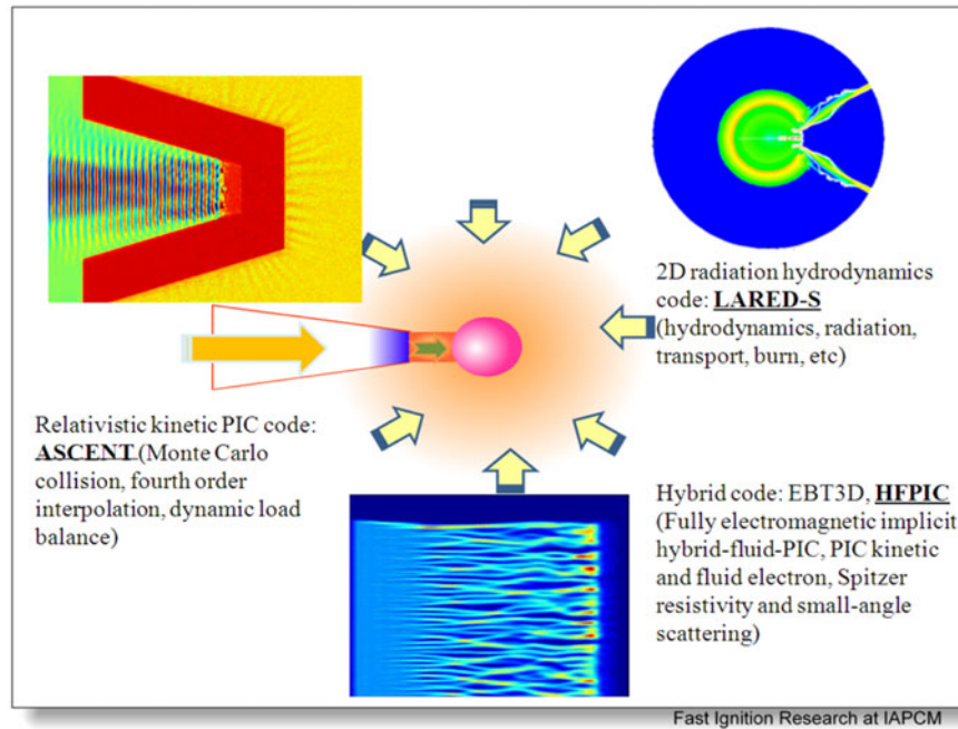
Figure 1. (Color online) A schematic diagram of the ICFI at the IAPCM.
