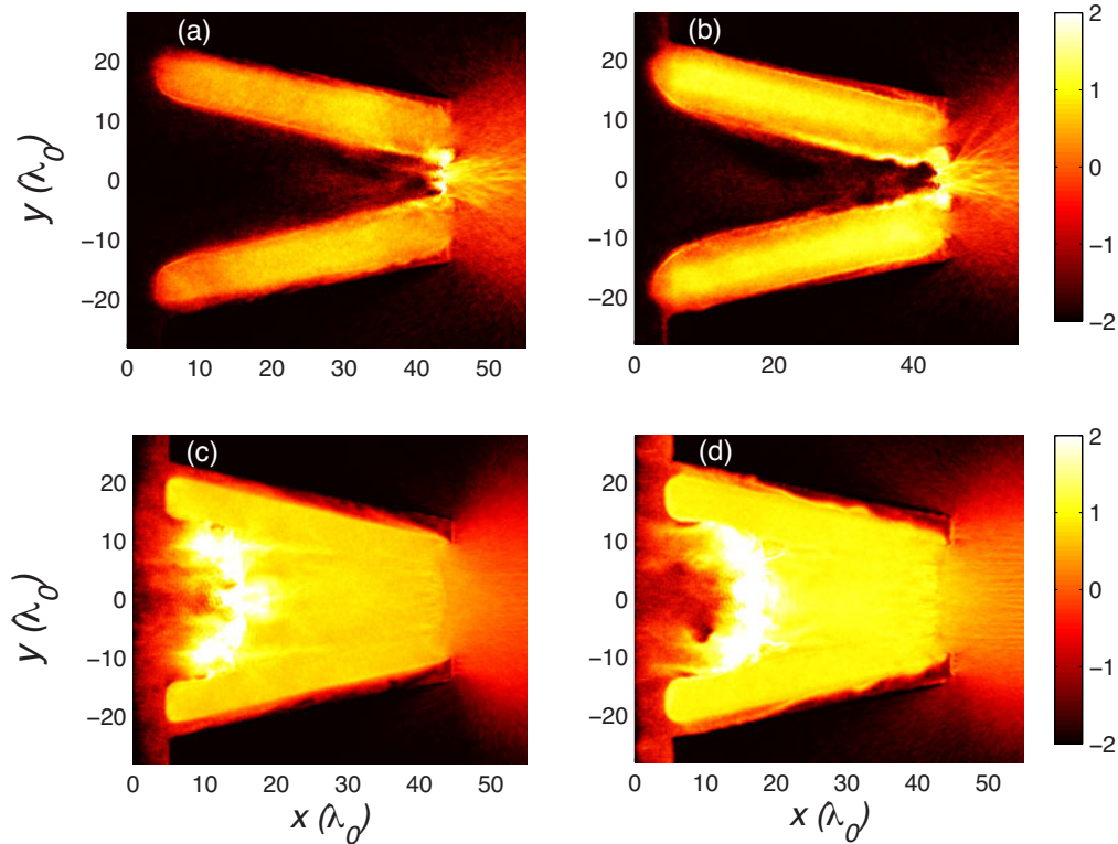
Figure 4. (Color online) The natural logarithm of the electron energy density for (a), (b) without and (c), (d) with large-scale preplasma at time (a), (c) t = 500 fs, and (b), (d) t = 1000 fs.
