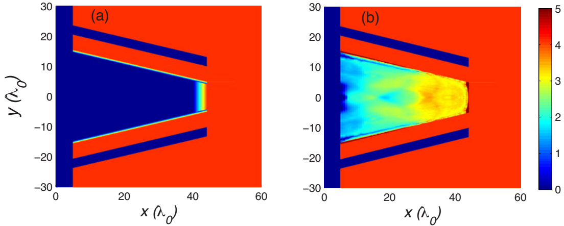
Figure 3. (Color online) Initial density profile of the double-cone target (a) without and (b) with large-scale preplasma.
