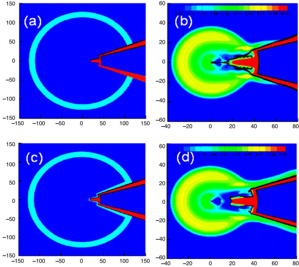
Figure 2. (Color online) Mass density contours of the cone-wire-in-shell target in LASER-S simulations. (a) and (b) are without the CH coating, (c) and (d) are with the CH coating. Black lines represent the contact surfaces between gold and the low-Z materials.
