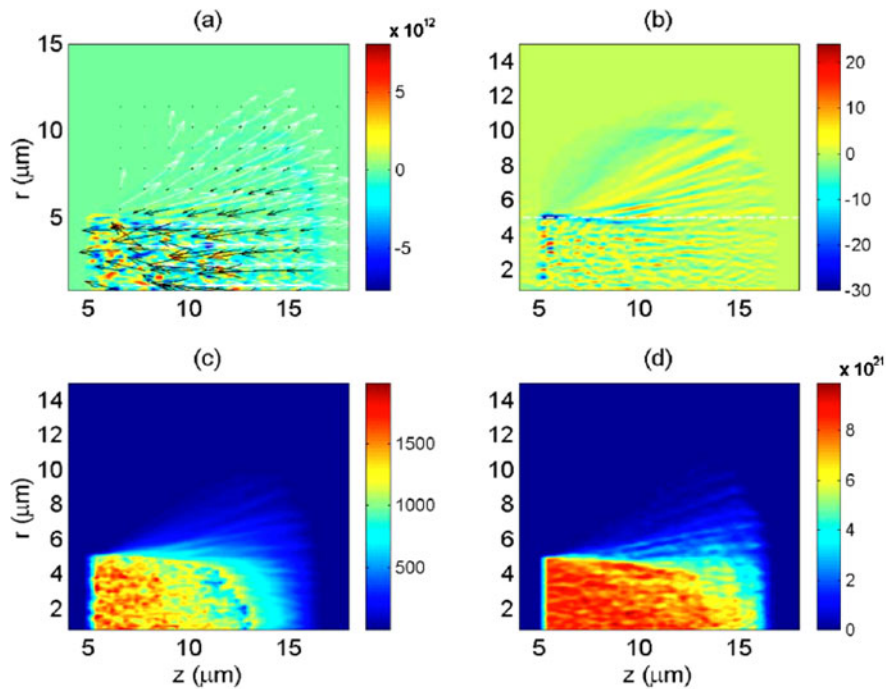
Figure 5. (Color online) Snapshots of (a) the longitudinal current density J_z(z, r) (in \text{A cm}^{-2} ), (b) the azimuthal magnetic B_\theta (in MG), (c) the temperature T_e (in eV) of the target plasma electrons, and (d) the beam density n_b (in \text{cm}^{-3} ) (from Zhou et al. 2008 [42] ).
