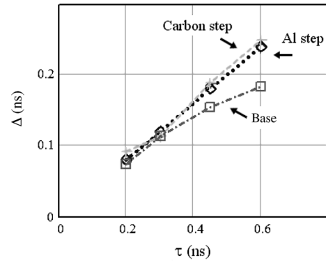
Figure 4. The dependences of the difference between shock arrivals for Gaussian pulses and the reference one (flat top) from \tau for all three parts of the target: (i) base (Al: 8 \mu\text{m} ); (ii) Al step (Al: 16.5 \mu\text{m} ); and (iii) carbon step (Al–C: 11.5 \mu\text{m} + 9.5 \mu\text{m} ) – \Delta_{\text{base}} , \Delta_{Al} and \Delta_C , correspondingly. All dependences are very close to each other for \tau \leq 300 ps.
