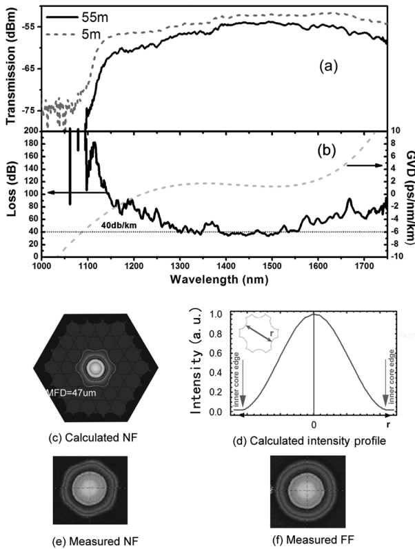
Figure 6. (a) The fibre optical transmission spectra measured by the white-light source for 55 m (solid curve) and 5 m (dotted curve). (b) The fibre optical attenuation spectrum (solid black curve) and GVD (dashed red line). The dotted horizontal line shows the baseline of the attenuation figure. (c) Calculated near-field (NF) pattern with an MFD of 47 \mu\text{m} . (d) Calculated intensity profile showing along the axis shown in the top-left inset. (e) Measured NF pattern showing an MFD of 46 \mu\text{m} . (f) Measured far-field (FF) pattern [32] .
