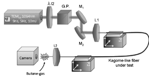
Figure 7. Experimental set-up for the laser-induced spark-ignition experiment. \lambda/2 : half wave plate @1064 nm, G.P.: Glan polarizer, M: mirrors, L: lenses [46] .
