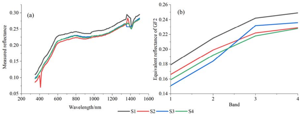
(a) 实测反射率 (a) Measured reflectance (b) GF2 传感器波段等效后的反射率 (b) Equivalent reflectance of GF2 sensor
