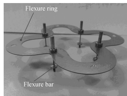
Fig.4 The flexure support of the FSM
