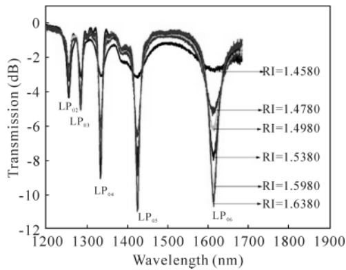
Fig.4 Transmission spectra of LPG with a period of 415 \mu\text{m} for different refractive indices of ambient higher than that of fiber cladding
