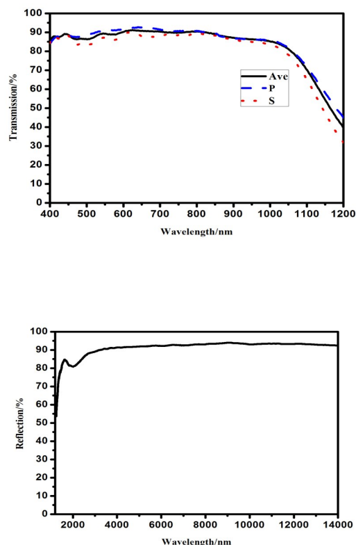
图9 分色片实测透/反射光谱曲线 Fig. 9 The measured transmission and reflection curves of the dichroic beam-splitter
