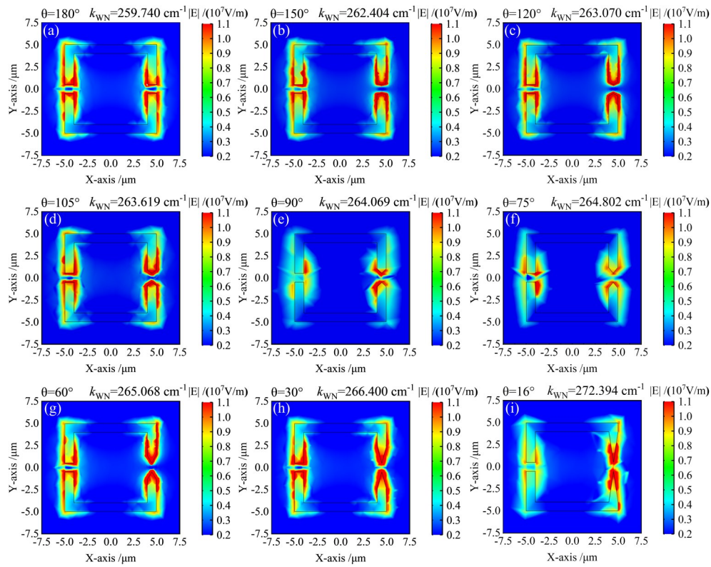
Fig. 3 Surface electric field distribution of far-IR metamaterial: (a) untipped structure; (b-i) asymmetric tip structure. The tip angle is (b) 150^\circ ; (c) 120^\circ ; (d) 105^\circ ; (e) 90^\circ ; (f) 75^\circ ; (g) 60^\circ ; (h) 30^\circ , and (i) 16^\circ , respectively
