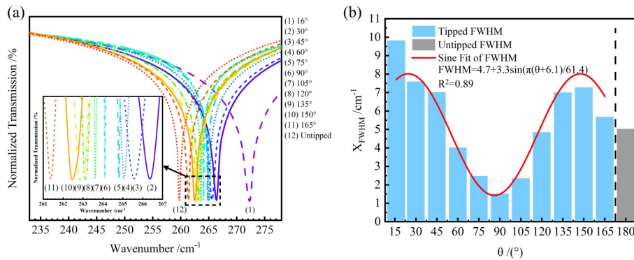
Fig. 5 FWHM under different asymmetric tip angles: (a) Normalized spectra; (b) Relationship between FWHM and tip angle. 图5 不同非对称针尖角度下超材料谐振峰的半峰宽:(a) 归一化谐振吸收谱;(b) 半峰宽与针尖角度之间的关系
