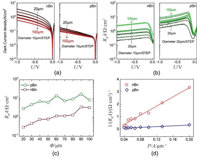
图3 20~100 \mu\text{m} 直径的nBn和pBn器件于室温下的(a)暗电流密度和电压变化曲线和(b) R_{\phi}A 随反向偏压的变化曲线;(c) 在400 mV反偏时,pBn和nBn器件 R_{\phi}A 随台面直径的变化;(d) (R_{\phi}A)^{-1} 与周长对面积( P/A )的变化曲线 Fig. 3 (a) Dark current density-voltage curves of nBn and pBn devices with diameters ranging from 20 \mu\text{m} to 100 \mu\text{m} at room temperature;(b) variation curves of R_{\phi}A with reverse bias;(c) R_{\phi}A varied with mesa diameters for pBn and nBn devices at a reverse bias of 400 mV;(d) variation of (R_{\phi}A)^{-1} over the perimeter-to-area ratio ( P/A )
