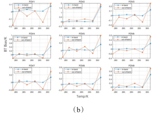
图8 不同探测元带内校正法和带外校正法的平均亮温偏差 (a)长波,(b)中波1 Fig. 8 Average brightness temperature deviations of medium-wave 1 by in-band and out-of-band correction methods of different FOV (a) LW, (b)MW1;
