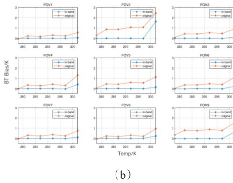
图7 不同探测元未校正和带内校正方法的平均亮温偏差 (a)长波,(b)中波1 Fig. 7 Average brightness temperature deviations of medium-wave 1 by uncorrected and in-band correction methods of different FOV (a) LW,(b)MW1
