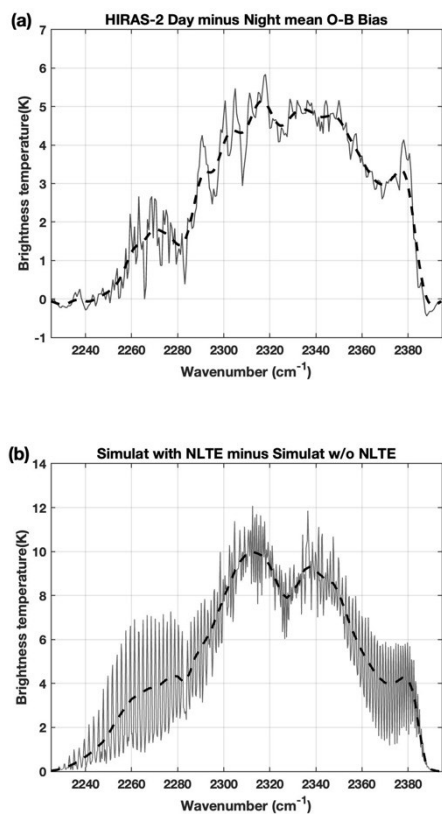
图8 非局地热力平衡效应,(a) HIRAS-II白天和黑夜O-B偏差的差和(b)IASI是否考虑NLTE效应对模拟亮温的影响 Fig. 8 Non-local thermodynamic equilibrium effect, (a) the difference between day and night HIRAS-II O-B deviation and (b) the influence of NLTE effect on IASI simulated brightness temperature
