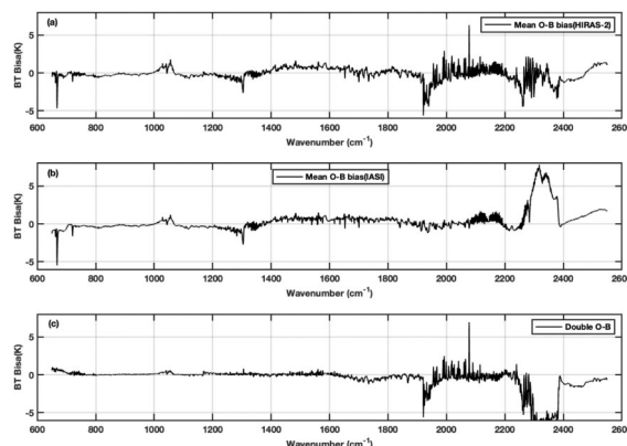
图9 偏差谱分布,(a) HIRAS-II,(b) IASI,(c) double O-B Fig. 9 The bias spectrum of (a) HIRAS-II, (b) IASI, (c) double O-B
