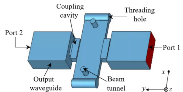
Fig. 2 The schematic drawing of the integrated-two-unit circuit with two output ports located on both sides of the two symmetrical coupling cavities
