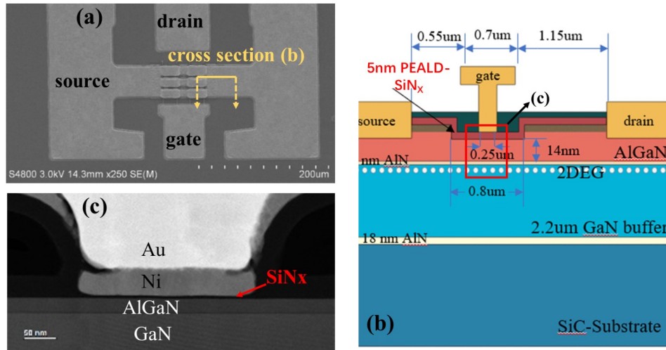
Fig. 1 Diagram of the AlGaN/GaN MIS-HEMT (a) SEM of 4 \times 50 \mu\text{m} device, (b) the schematic of epitaxial structure, (c) TEM of 0.25\text{-}\mu\text{m} T-gate
