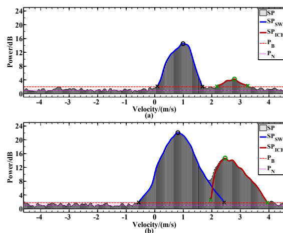
图3 那曲2015年8月2日23:22雷达在层积云2.7 km和2.91 km探测的功率谱,(a)和(b)分别为多模态和多谱峰现象, SP 、 SP_{sw} 和 SP_{ice} 分别为原始谱和分离的过冷水和冰晶谱 Fig. 3 Radar Doppler spectra detected at 23:22 on August 2, 2015 over Nagqu at 2.7 km and 2.91 km of the stratocumulus, (a) and (b) reflect phenomena of multiple modals and multiple peaks, SP , SP_{sw} , and SP_{ice} represent the original spectra, supercooled water spectra, and ice crystal spectra
