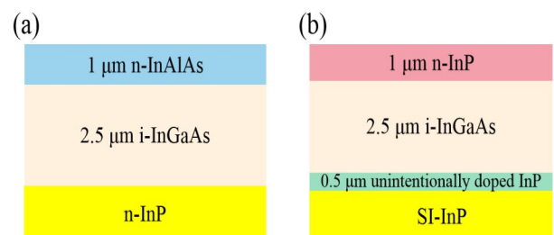
图 1 (a) \text{In}_{0.81}\text{Ga}_{0.19}\text{As}/\text{In}_{0.81}\text{Al}_{0.19}\text{As} 探测器结构示意图, (b) \text{In}_{0.53}\text{Ga}_{0.47}\text{As}/\text{InP} 探测器结构示意图
