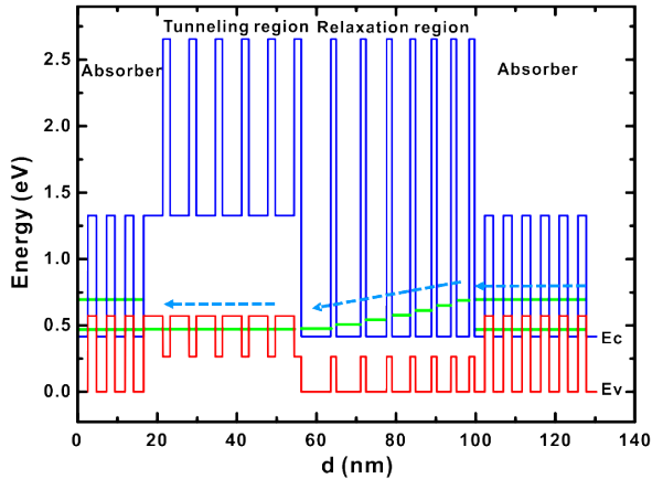
图1 带间级联探测器能带结构示意图,箭头表示电子运动方向,绿色线表示超晶格和量子阱中电子或者空穴能级位置 Fig. 1 The energy band alignments for the ICIP, the arrow shows the transport direction of the electron, and the green lines shows the energy level for the electron or holes in the superlattices and quantum wells
