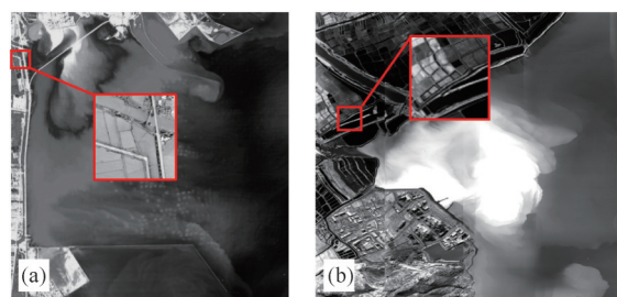
图 19 温排水检测影像分辨率对比: (a)SIRI-4 红外影像细节, (b)MAMS 红外影像细节 Fig. 19 Image resolution comparison of thermal drainage detection: (a) infrared image details of SIRI-4, (b) infrared image details of MAMS
