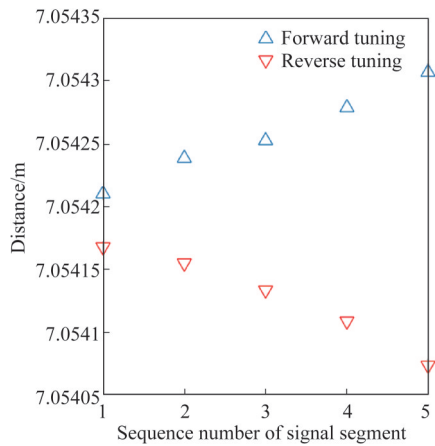
Fig. 4 Ranging value of the measured signal in different sections 图4 测量信号不同段的测距值
