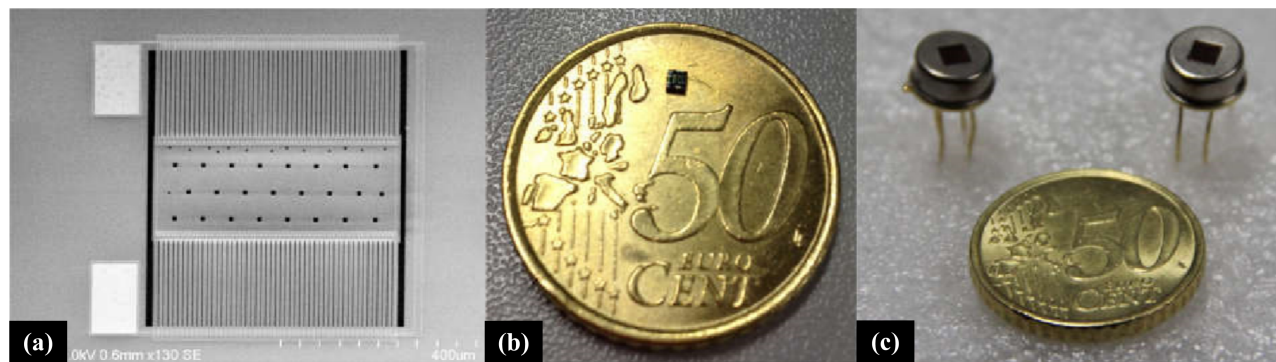
图2 MEMS热电堆红外探测器:(a)芯片电镜图;(b)裸芯片;(c)封装后器件 Fig. 2 MEMS thermopile IR detector:(a) SEM image of chip; (b)Bare chip; (c)Packaged detector
