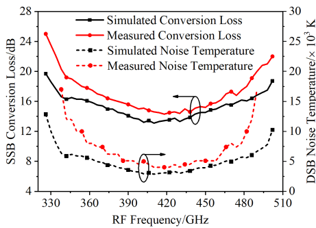
Fig. 12 Comparison between simulated conversion loss and measured results of the proposed mixer with fixed IF frequency of 1 GHz and optimum LO power of 7 mW 图 12 在1GHz固定中频和7mW最优本振功率下,混频器仿真和测试的变频损耗的对比
