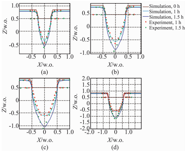
图6 1#样品中不同名义沟槽宽度的碲镉汞及光刻胶刻蚀轮廓的实验结果和计算结果. 轮廓中 Z > 0.5 的部分为掩膜, Z \leq 0.5 的部分为碲镉汞. (a) 4 μm, (b) 6 μm, (c) 8 μm, (d) 10 μm Fig. 6 Comparison between simulated profiles and experimental profiles of 1# sample. On these profiles the zone where Z > 0.5 is mask, the zone where Z \leq 0.5 is HgCdTe. (a) 4 μm, (b) 6 μm, (c) 8 μm, (d) 10 μm
