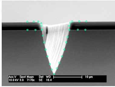
图5 1#样品中名义沟槽宽度为8 μm的刻蚀轮廓的提取,图中绿色圆圈代表在刻蚀轮廓上提取的离散点 Fig. 5 The extraction of etching profile of 1# sample with 8 μm nominal trench width from the scanning electron micrograph, the green circles are used to represent discrete points on the etching profile
