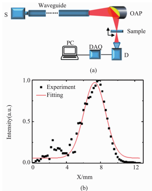
图 4 (a) 太赫兹波透射成像系统示意图, (b) 焦点处太赫兹光斑大小 Fig. 4 (a) Schematic of terahertz wave transmission imaging system, (b) Terahertz spot size at the focal point
