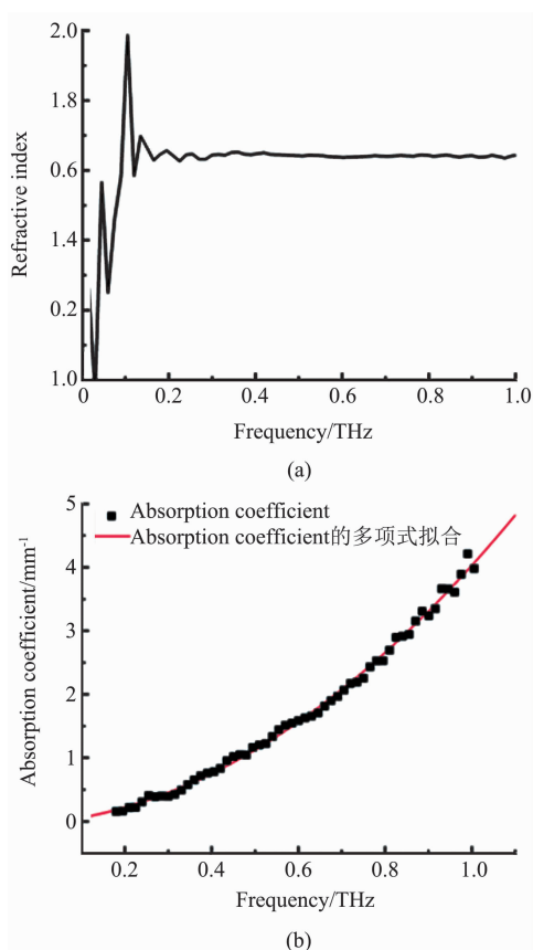
图1 PLA材料参数表征:(a) PLA材料的折射率,(b) PLA材料的吸收系数 Fig. 1 Characteristics of PLA polymer:(a) Refractive index of PLA,(b) Absorption coefficient of PLA
