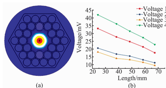
图3 (a) 仿真纤芯基模场分布;(b) 实测波导损耗 Fig. 3 (a) Simulated core fundamental mode distribution;(b) The experimental waveguide loss
