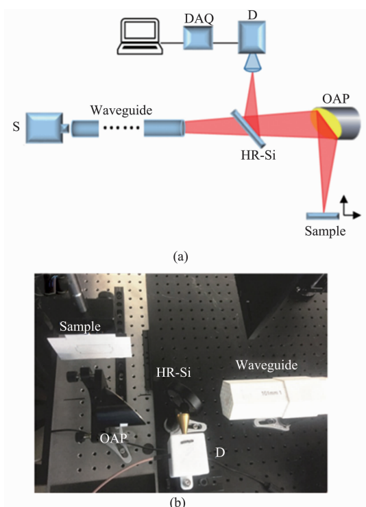
图 7 太赫兹波反射成像系统: (a) 示意图, (b) 实物图 Fig. 7 Terahertz wave reflection imaging system: (a) Schematic diagram, (b) Photograph of reflection imaging system
