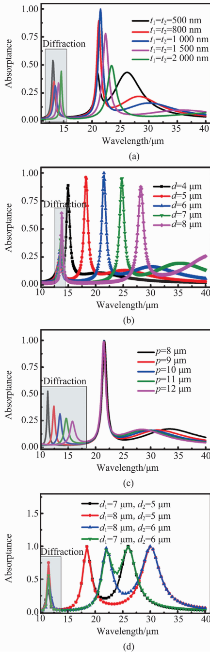
Fig. 4 The simulated absorbance as a function of wavelength and the thickness of dielectric layer (a), the side lengths of gold particle (b), the periods of gold particle (c) for this double-resonant layer absorber (d) Absorption spectrum of varying the side lengths of gold particle at the top and bottom layers
