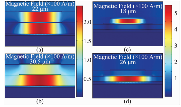
Fig. 5 (a) and (b) are the magnetic field distribution profile corresponding to the the incident wavelength of 22 \mu\text{m} and 30.5 \mu\text{m} , respectively, for the double-resonant layer absorber with t_1 = t_2 = 1000 \text{ nm} , d_1 = d_2 = 6 \mu\text{m} , and p = 10 \mu\text{m} ; (c) and (d) are the magnetic field distribution profile corresponding to the the incident wavelength of 18 \mu\text{m} and 26 \mu\text{m} , respectively, for the double-resonant layer absorber with t_1 = t_2 = 1000 \text{ nm} , d_1 = 7 \mu\text{m} and d_2 = 5 \mu\text{m} , and p = 10 \mu\text{m}
