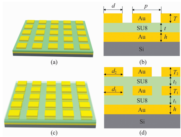
Fig. 1 (a) and (c) are the schematic structure for the metamaterial perfect absorbers with single-resonant cavity and double-resonant cavities respectively, (b) and (d) are the respective cross-sectional profiles for structure (a) and (c)
