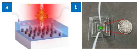
(a) Schematic diagram of optofluidic sensor; (b) Physical diagram of optofluidic sensor
