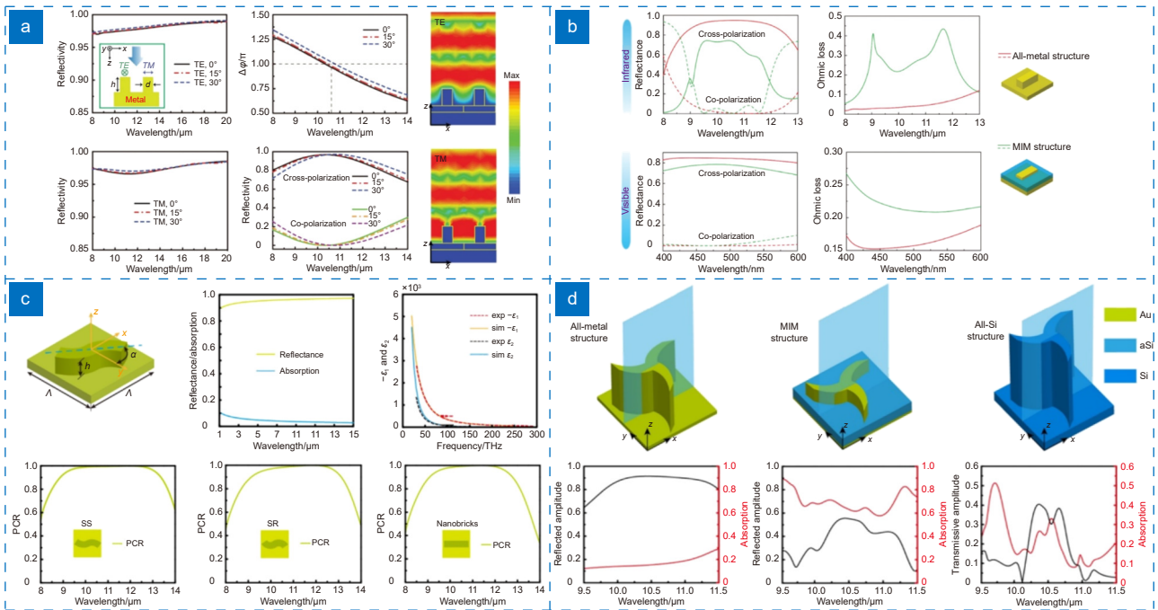
图 2 不同金属单元结构的仿真结果。(a) 金属光栅的仿真结果 [36] ；(b) 金属纳米砖的仿真结果及其与 MIM 结构的对比 [37] ；(c) S 型单元结构的仿真结果 [47] ；(d) 不同 C3 结构的仿真对比 [50] Fig. 2 Simulation results of different metal unit structures. (a) Simulation results of metal gratings [36] ；(b) Simulation results of metal nanobricks and comparison with MIM-type structure [37] ；(c) Simulation results of S-type unit structure [47] ；(d) Simulation comparison of different C3 structures [50]
