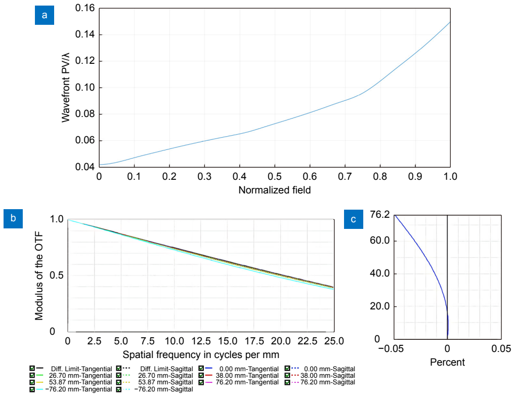
图 11 干涉仪成像光路像质评价。(a) 归一化视场成像波前 PV; (b) MTF 曲线; (c) 畸变曲线 Fig. 11 Image quality evaluation of the interferometer imaging optical path. (a) Imaging wavefront PV of the normalized field; (b) MTF curve; (c) Distortion curve
