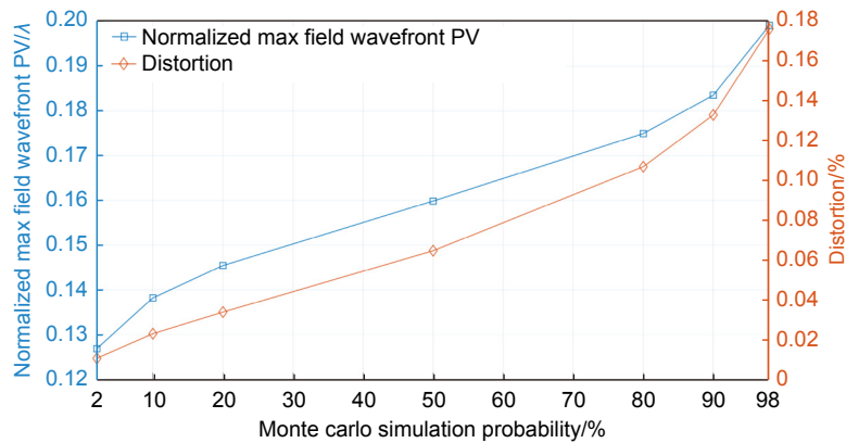
图 12 干涉仪成像光路蒙特卡罗模拟公差分析 Fig. 12 Monte carlo simulation tolerance analysis of the interferometer imaging optical path
