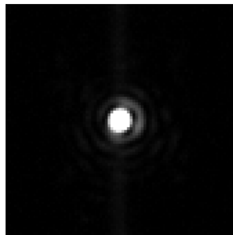
Fig. 6 PSF corrected by using J_0
