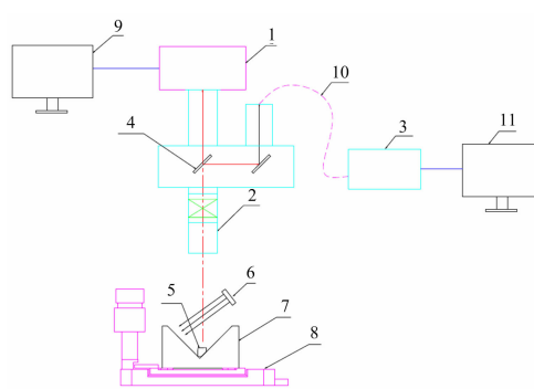
Fig. 1 Instrument working principle diagram
