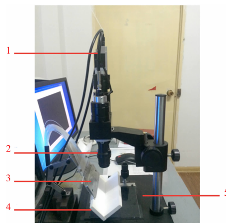
Fig. 2 Experimental device diagram
