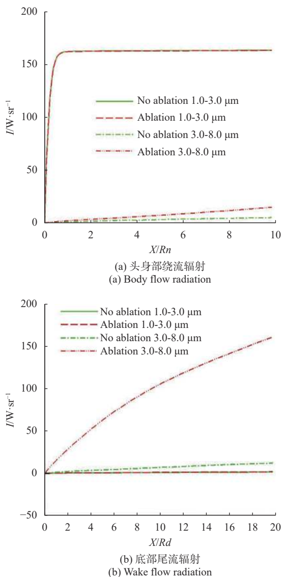
图 5 烧蚀效应对再入体头身部绕流与底部尾流积分辐射强度的影响 Fig.5 Effects of ablation products on radiation intensity of flow over reentry body with base wake
