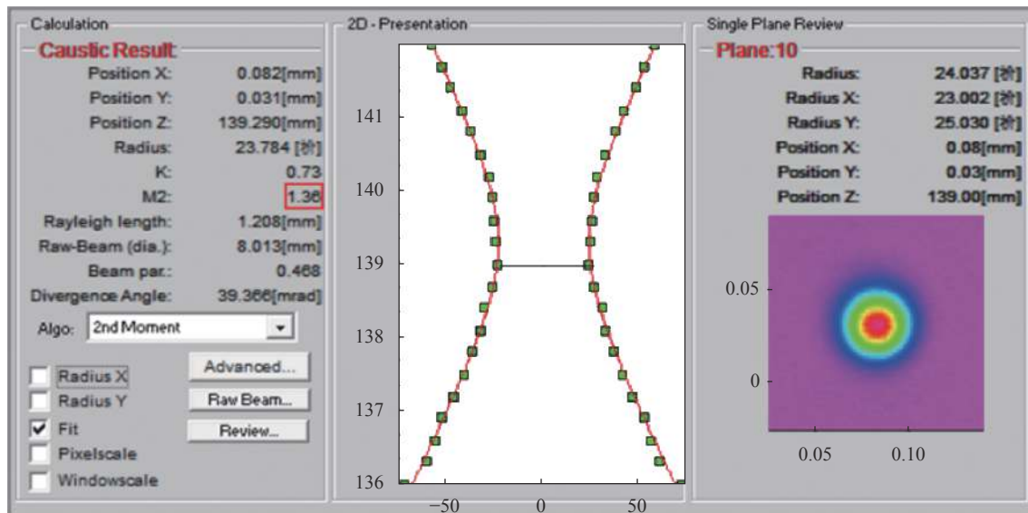
(c) M^2=1.36
