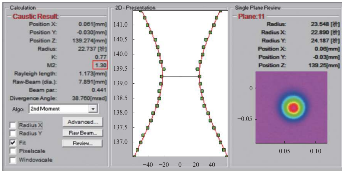
(b) M^2=1.30
