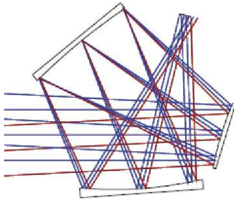
(c) 完全倾斜 (c) Fully tilted
