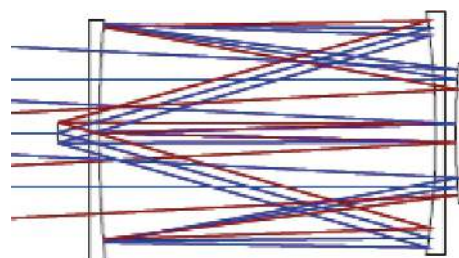
(a) 同轴光学系统 (a) On-axis optical system
