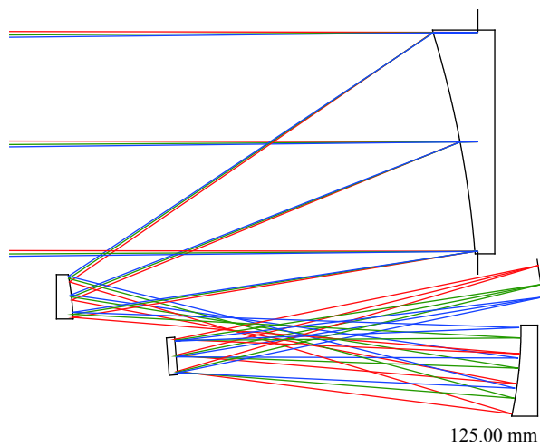
图 26 “天问一号”高分辨率相机光学系统 Fig.26 Optical system of high resolution imaging camera on “Tianwen-1” mission
