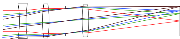
图 24 反摄远透镜光学系统 Fig.24 Inverse telephoto optical system
