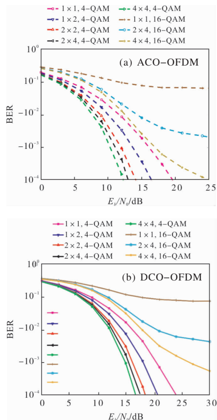
Fig.3 BER for the optical OFDM 4–QAM and 16–QAM constellations in a turbulence channel with \sigma_l^2=0.2
