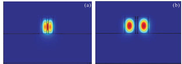
图 3 (a)狭缝波导基模 \text{TE}_0 ;(b)狭缝波导一阶高阶模式 \text{TE}_1 Fig.3 (a) \text{TE}_0 mode of the slot waveguide; (b) \text{TE}_1 mode of the slot waveguide
