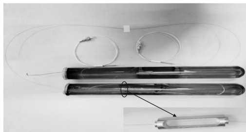
Fig.6 Packaged LPG temperature sensor
