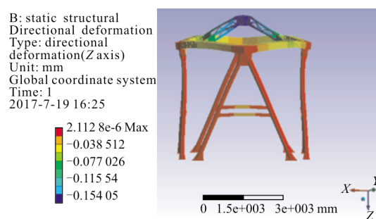
(a) 光轴竖直 (a) Vertical optical axis
