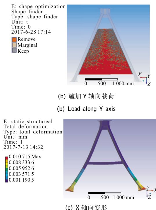
(c) X 轴向变形 (c) Deformation along X axis
