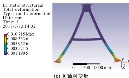
(c) X 轴向变形 (c) Deformation along X axis
