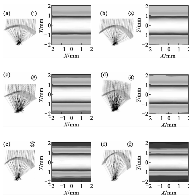
Fig.11 Illumination distribution of the six curved Fresnel lenses
