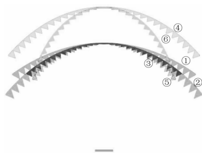
Fig.10 Shape of the six Fresnel lenses
