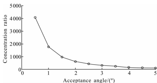
Fig.9 Relation between acceptance angle and concentration ratio
