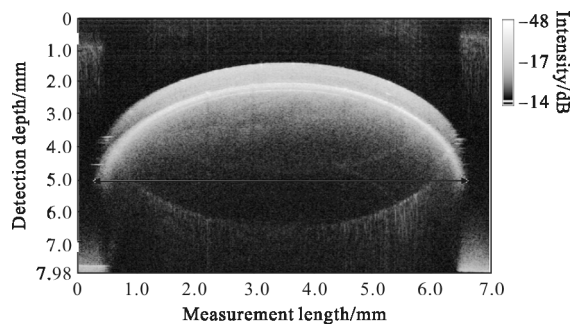
(e) 珍珠样品 OCT 直径测量示意图 (e) Images of pearl diameter measured by OCT
