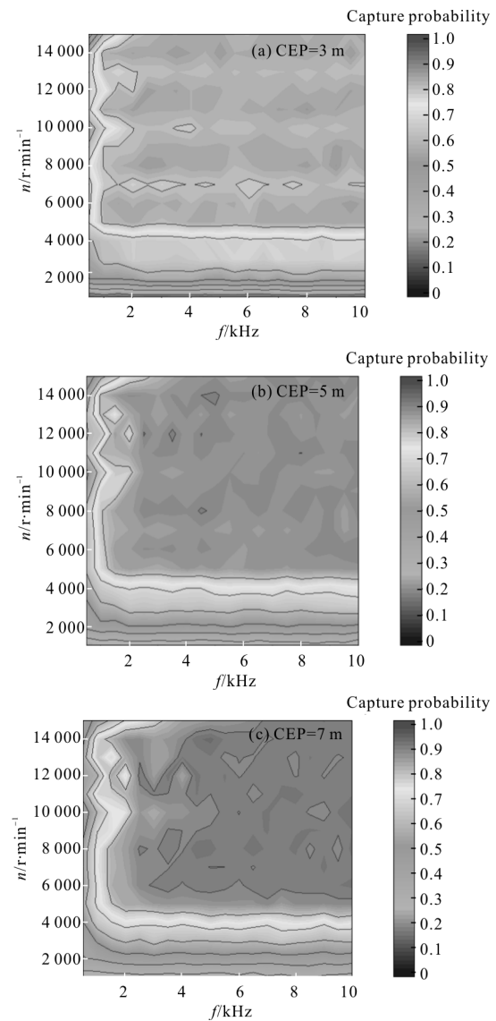
图 12 不同命中精度下采用激光周向探测系统时的捕获概率 Fig.12 Target capture probabilities of laser circular viewing detection system under different hit accuracy
