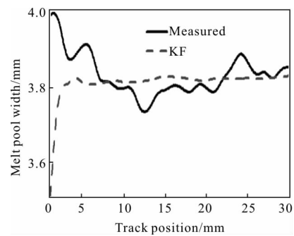
图 5 熔池宽度测量值及卡尔曼滤波值 Fig.5 Plots of measured and KF filtered melt pool width
