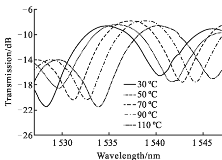
Fig.7 Spectrum of the two spherical-shape structures MZI at different temperature
