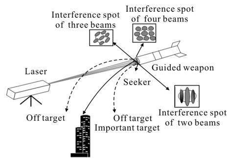
图 1 准平行光干涉的激光干扰方案示意图 Fig.1 Schematic diagram of quasi parallel light interference laser jamming scheme
