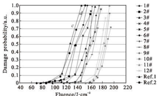
图 5 不同预处理参数下的 150 发次损伤形态转化几率曲线 Fig.5 Curves of damage morphology change probability under 150 pulse with varied laser conditioning parameters
