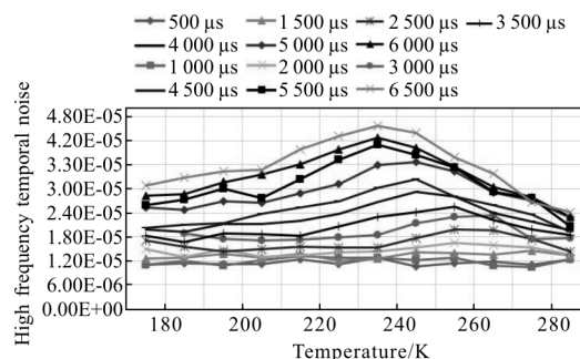
图 4 高频时间噪声和黑体温度、积分时间的关系 Fig.4 Relations of high frequency temporal noise, blackbody temperature and integration time
