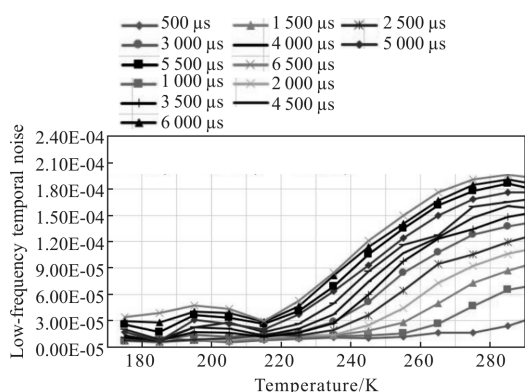
图 3 低频时间噪声和黑体温度、积分时间的关系 Fig.3 Relations of low-frequency temporal noise, blackbody temperature and integration time
