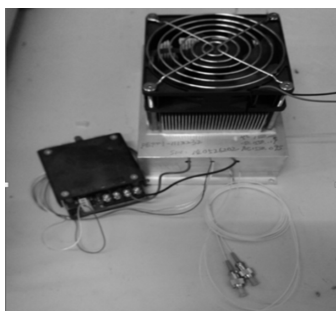
Fig.3 Physical map of etalon with temperature control module
