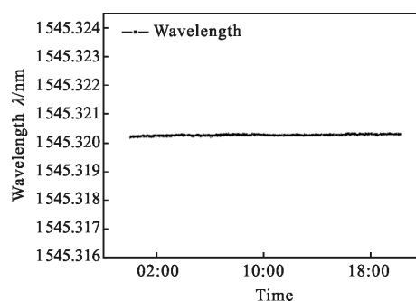
(a) FBG wavelength demodulation system
