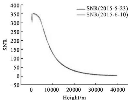
图 4 激光雷达信噪比廓线 Fig.4 Profile of SNR of lidar
