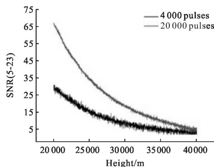
图 7 脉冲累积的 SNR 对比图 Fig.7 Comparison of SNR based on pulse accumulation method
