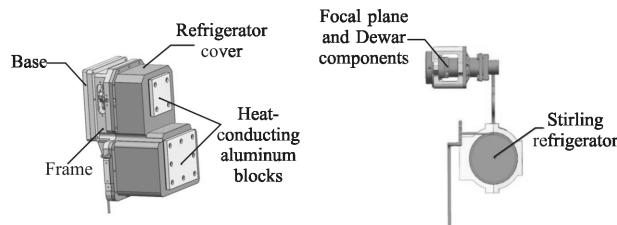
(a) 红外探测器组件外部结构 (b) 红外探测器组件内部结构 (a) Exterior structure of infrared detectors (b) Interior structure of infrared detectors
